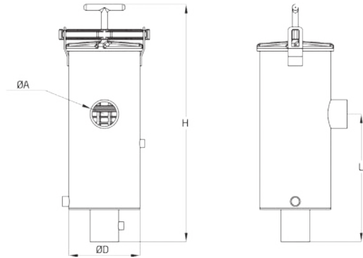
Angle Type dic-screen filter (L-D 3000 series)
