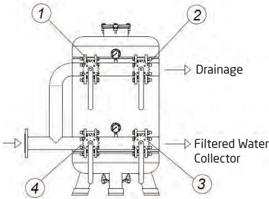
Back-Flushing Mode: 2,4: Open - 1,3: Closed
