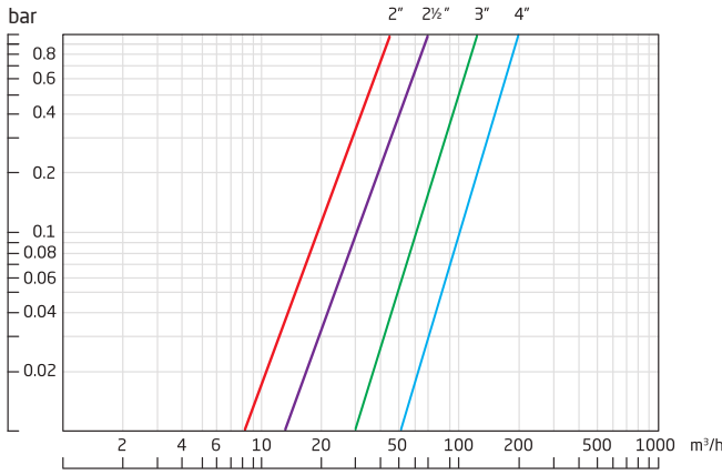
Angle Type disc-screen filter (L-D 3000 series)
