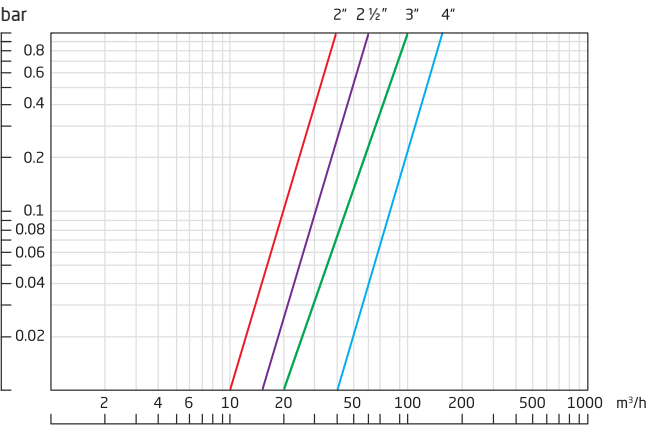
Y Type disc-screen filter (Y-D 3000 series)
